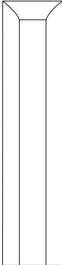
Straight Splash Block 36" L. x 10 1/2" W. x 2 1/2" H. Stock Pricing Depends on Quantity
